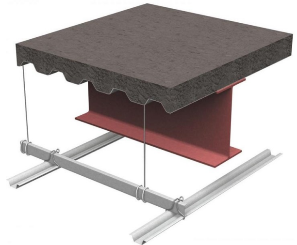
Hanger Wire used a in drop ceiling application
